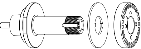
GWA manual HSK-F40 // ø20 mm // without RS
